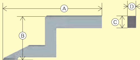
■ Scriber for SHT-1-J : Dimensions (Unit : mm)
