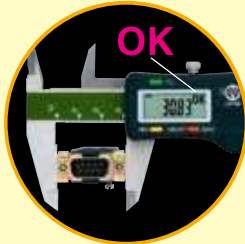
Judgment function
